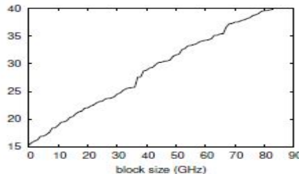
Fig. 3. The median response time of Pice, compared with the other frameworks [28].
